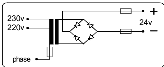
Connecting diagram
