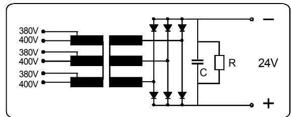
Connecting diagram
